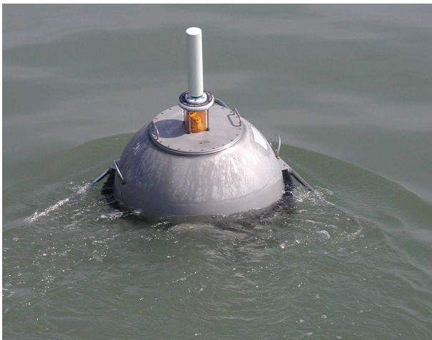
Figure 2: Waverider Buoy
